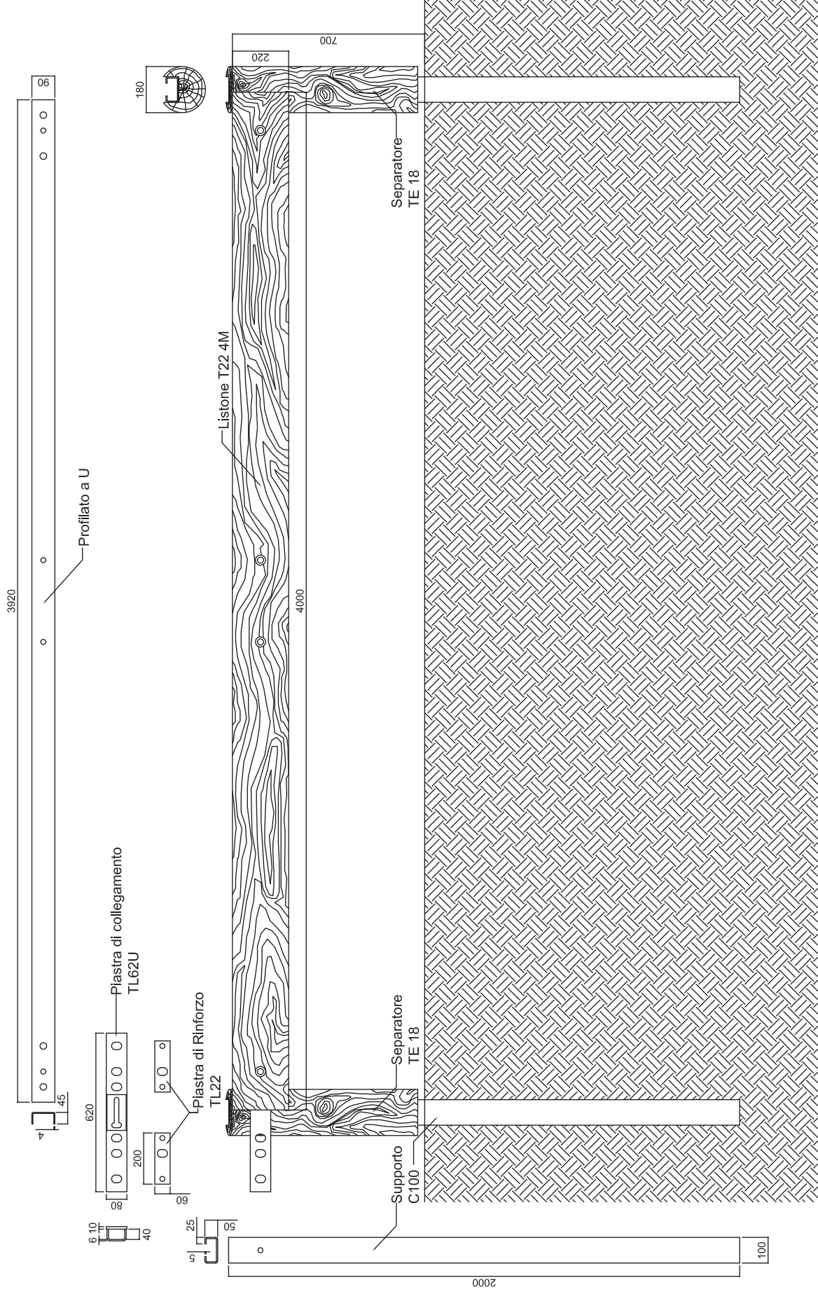
Metal Wood srl - Barriera Stradale T22 4m
